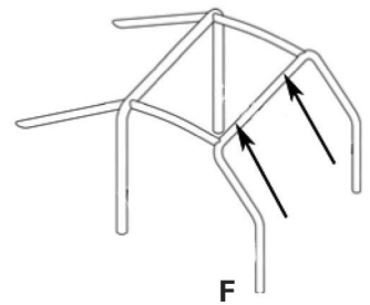
F Roof attachment (front)
