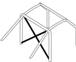
N X brace on main hoop dwg. 253-7
