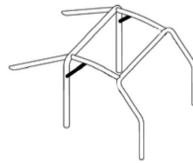
K Rear hoop reinforcements dwg. 253-31
