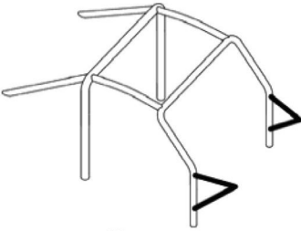
C Front turret attachment dwg. 253-25
