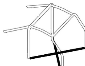
P X brace on floor dwg. 253-31
